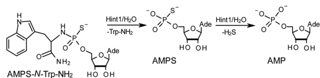
Scheme 3 The HINT1 catalyzed hydrolysis of adenosine-5'-O-((L-tryptophan amide-N α -yl)-phosphoramidothioate) (AMPS-Trp-NH 2 ), followed by desulfuration of the AMPS intermediate leading to the formation of adenosine-5'-O-phosphate.
