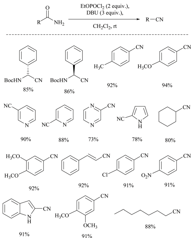
Scheme 13 Ethyl dichlorophosphate as a dehydrating agent.
