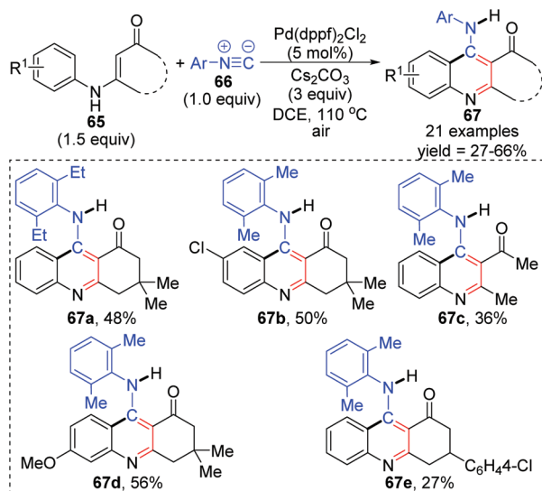
Scheme 15 Synthesis of 4-aminoquinoline derivatives via 1,3-palladium migration.
