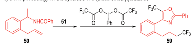
Fig. 10 Phosphine-catalyzed bistrifluoromethylation of allylphenyl amide.
