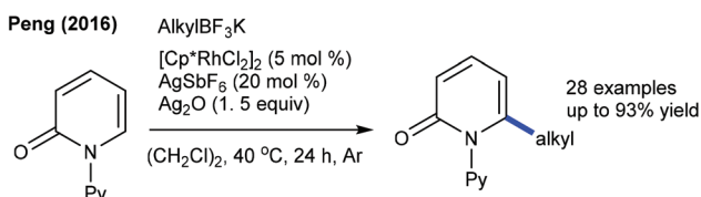
Scheme 48 C6-Alkylation of pyridones.
