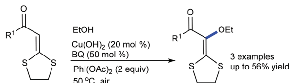
Scheme 148 Ethoxylation of cyclic \alpha -aryalketene dithioacetal.
