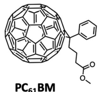
Fig. 5 Chemical structures of P3HT , PCDTBT , PSBTBT , DPP-SVS , PNDI-TV , PC 61 BM , PC 71 BM and ICBA .
