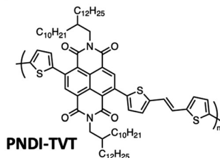
Fig. 5 Chemical structures of P3HT , PCDTBT , PSBTBT , DPP-SVS , PNDI-TV , PC 61 BM , PC 71 BM and ICBA .
