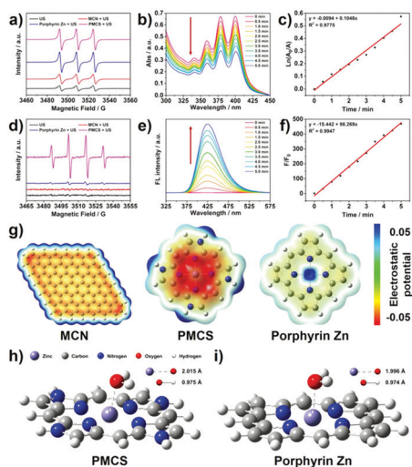
Fig. 5 In vitro ROS generation abilities of PMCS upon exposure to ultrasound (a–f). (g) The electrostatic potential profiles of different molecules. (h and i) Molecular models of adsorbed \text{H}_2\text{O} on PMCS and porphyrin Zn. Reproduced with permission ref. 63.
