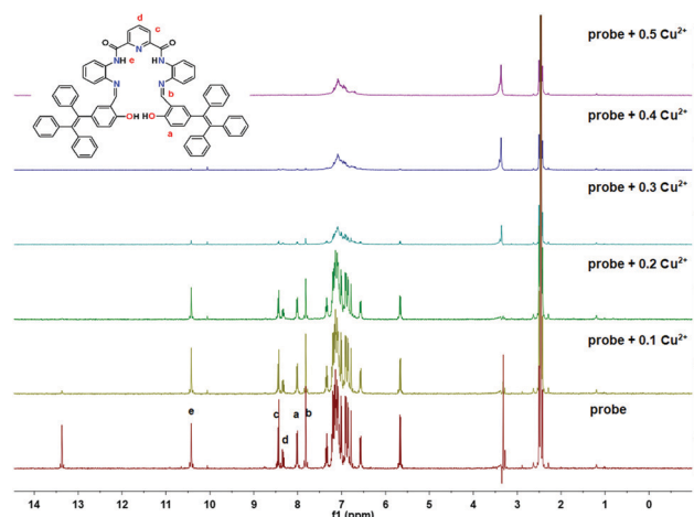
Fig. 6 ^1\text{H} NMR spectroscopic titration spectra of probe@Cu 2+ on increasing concentrations of \text{Cu}^{2+} in \text{d-DMSO} solution.
