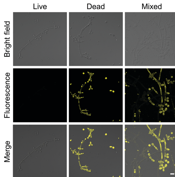
Fig. 3 The confocal laser scanning microscope (CLSM) images of C. albicans stained with 10 \mu\text{M} DPASI. \lambda_{\text{ex}} = 488 nm; scale bar = 10 \mu\text{m} .
