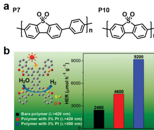
Fig. 19 (a) Structures of the liner polymers P7 and P10. (b) HER of the DBTD-CMP1 photocatalyst under different conditions. Reproduced from ref. 151 with permission from the American Chemical Society, Copyright 2018.
