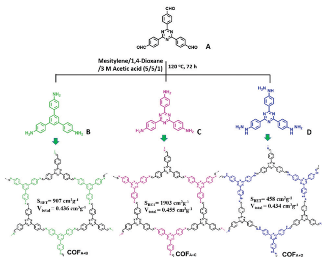
Fig. 14 Synthesis and structures of \text{COF}_{\text{A+B}} , \text{COF}_{\text{A+C}} and \text{COF}_{\text{A+D}} . Modified from ref. 135 with permission from Elsevier, Copyright 2018.
