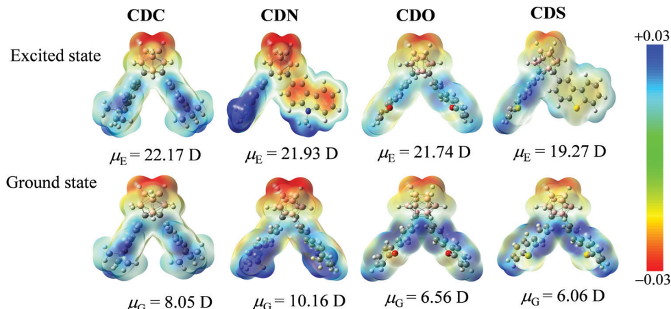
Fig. 10 Electrostatic potential of CDC, CDN, CDO and CDS at 0.001 a.u. isosurface of electron density by (TD-) DFT computed at the B3LYP/6-31G(d,p) level in the ground ( \mu_G ) and excited ( \mu_E at the Franck–Condon geometry) dipole moments (blue color indicates electron-rich, red color indicates electron-deficient).
