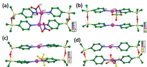
Fig. 17 The solid-state structures of (a) 23 ; (b) 24 ; (c) 25 ; (d) 26 showing transannular \text{Ag} - \text{Ag} interactions. The anions can be clearly observed, and hydrogen atoms are removed for clarity.
