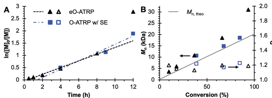
Fig. 3 Plot of the natural logarithm of monomer ( M ) consumption over time (A). Molecular weight (filled markers) and D (hollow markers) evolution (B) for eO-ATRP (black triangles) and O-ATRP with supporting electrolyte (blue squares). Conditions: [MMA] : [DBMM] : [1] = [1000] : [5] : [0.1], 2 mL MMA, 2 mL DMAc, SE = 0.094 M \text{Bu}_4\text{NPF}_6 and 0.006 M \text{Bu}_4\text{NBr} . Reactions performed in a U-cell and irradiated with a high-power white LED (see Experimental equipment in ESI†). For eO-ATRP, working electrode = glassy carbon, counter electrode = Pt wire, reference electrode = Ag wire quasi-reference electrode, and E_{\text{app}} = E_{1/2} - 120 mV.
