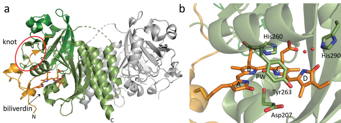
Fig. 3 Overview structure and chromophore binding of the BphP PAS-GAF fragment. (a) The structural features of a PAS-GAF dimer from Deinococcus radiodurans phytochrome (DrBphP, PDB id 6T3L 95 ). Subunit 1 with its PAS and GAF domain is colored in different shades of green whereas subunit 2 is grey. N-Terminal end of the PAS domain as well as biliverdin chromophore are colored in orange. The biliverdin position and knot region are indicated. (b) Zoom in on the biliverdin and selected surrounding amino acid residues. Residue numbers are from DrBphP, and the ring names (A–D) are indicated. The so-called pyrrole water (PW) and two well-defined waters between His290, biliverdin D-ring, and C-ring propionate group are also shown as red spheres (PDB id: 4Q0H 96 ).
