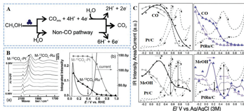
Fig. 1 (A) MOR reaction pathways. Reproduced with permission from ref. 81. Copyright 2006, American Chemical Society. (B) In situ ATR-SEIRAS of preadsorbed \text{M-}^{13}\text{CO}_{\text{L}} on the Ru/Pt ( \text{M-}^{13}\text{CO}_{\text{L}} refers to the linearly bonded CO generated by methanol), and the integrated IR intensity of the \text{M-}^{13}\text{CO}_{\text{L}} -Pt and \text{M-}^{13}\text{CO}_{\text{L}} -Ru as a function of electrode potential. Reproduced with permission from ref. 82. Copyright 2015, John Wiley & Sons Ltd. (C) \text{CO}_{\text{ads}} and \text{CH}_3\text{OH}_{\text{ads}} band integrals as a function of potential in both positive and negative scans on Pt/C and PtRu/C, respectively. Reproduced with permission from ref. 84. Copyright 2012, Royal Society of Chemistry.
