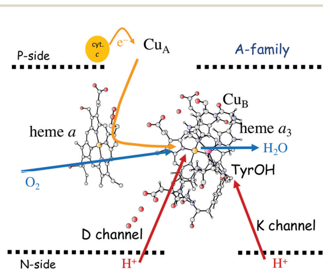
Fig. 10 Active site of the a_3A family oxidases showing the two proton channels from the N-side of the membrane to the active site. The D channel ends near the center of the BNC and the K channel ends at the redox-active tyrosine. The B and the C families have only one proton channel, the K analogue, located in a similar position as the K channel.
