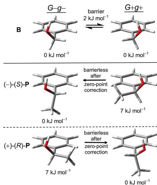
Fig. 2 G-g- and G+g+ monomer conformers of B , (-)\text{-(S)-P} and (+)\text{-(R)-P} with relative zero-point corrected energies and interconversion barriers at B3LYP-D3 level.
