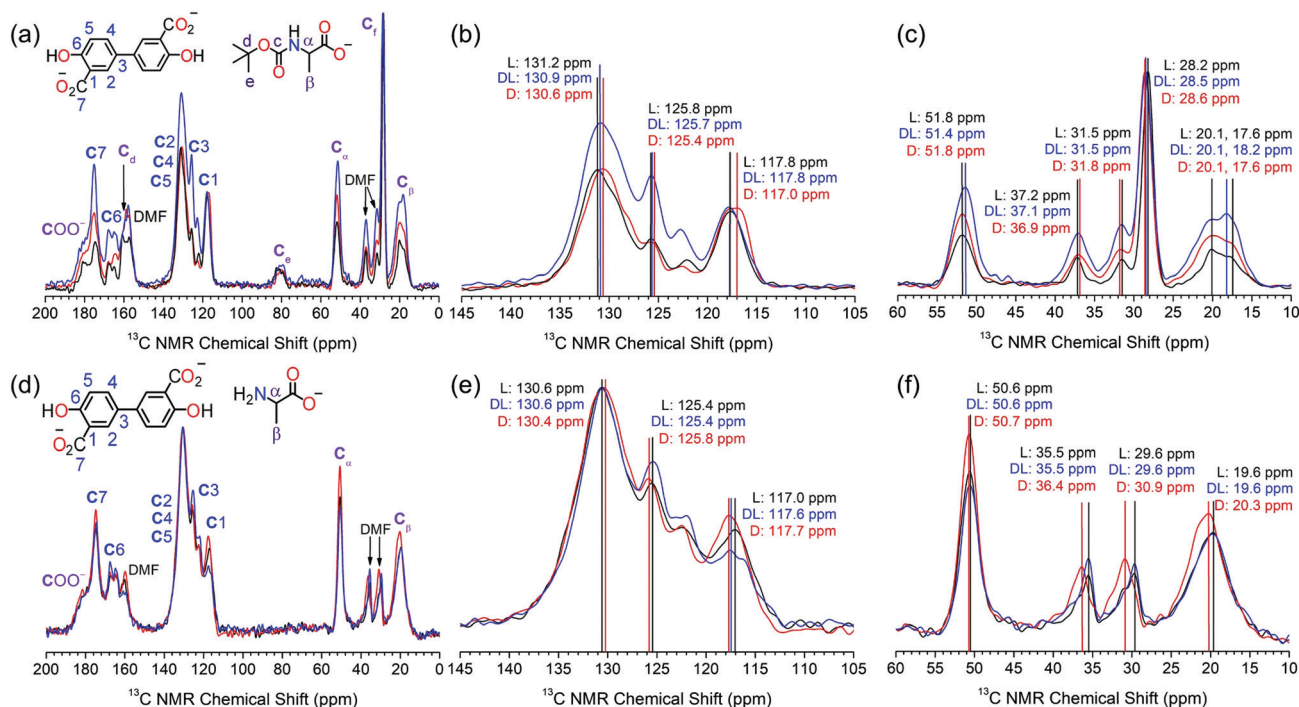
Fig. 2 ^{13}\text{C} solid state CPMAS spectra of \text{Mg}_2\text{dobpdc} @BOC-L-Ala (black), \text{Mg}_2\text{dobpdc} @BOC-D-Ala (red) and \text{Mg}_2\text{dobpdc} @BOC-DL-Ala (blue) acquired at 175 MHz showing (a) the full spectrum between 200–0 ppm, (b) zoomed in section between 145–105 ppm, and (c) zoomed in section between 60–10 ppm. The ^{13}\text{C} solid state CPMAS spectra of \text{Mg}_2\text{dobpdc} @L-Ala (black), \text{Mg}_2\text{dobpdc} @D-Ala (red) and \text{Mg}_2\text{dobpdc} @DL-Ala (blue) acquired at 175 MHz showing (d) the full spectrum between 200–0 ppm, (e) zoomed in section between 145–105 ppm, and (f) zoomed in section between 45–10 ppm. All spectra are scaled to the same maximum intensity.
