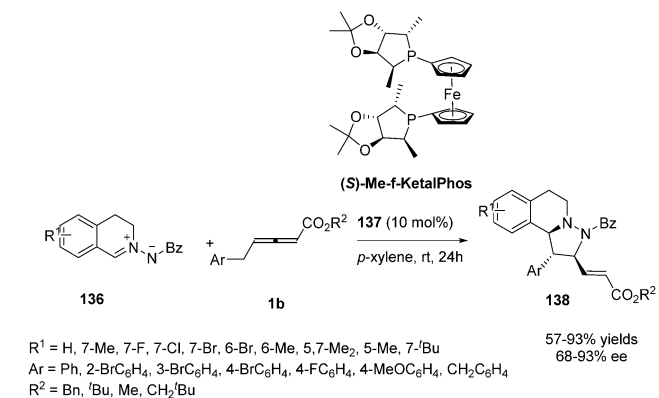
Scheme 44 Chiral phosphine-catalysed asymmetric (3+2) annulations of \gamma -substituted allenates.
