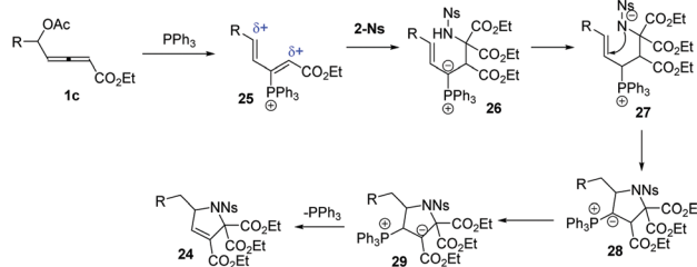
Scheme 8 Plausible mechanisms.
