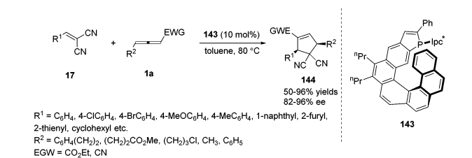
Scheme 46 Phosphahelicene catalysed (3+2) cyclizations of \gamma -substituted allenates and electron-poor olefins.
