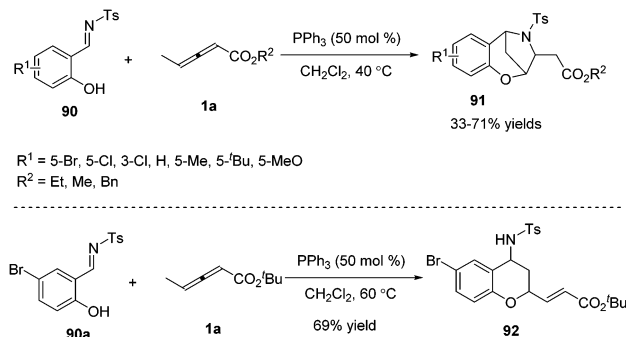
Scheme 29 PPh 3 -Catalysed sequential annulation reactions between salicyl N -tosylimines and allenates.
