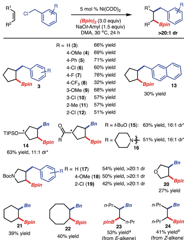
Scheme 3 Substrate scope.
