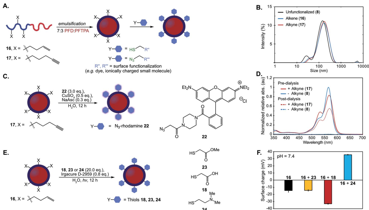
Fig. 4 (A) Schematic of post-emulsion modification strategy (with surfactants 16 and 17 ). (B) Dynamic light scattering data of emulsions formed from 8 , 16 , 17 . Emulsions were prepared with 10 vol% 7 : 3 PFD/PFTPA and 2.8 wt% surfactant in PBS, diluted 1 : 100 in MilliQ water and analyzed via DLS. (C) CuAAC chemistry is employed for emulsion surface functionalization with azidorhodamine dye 22 (NaAsc = sodium ascorbate). (D) Emulsions formed from 8 and 17 were subjected to the CuAAC chemistry conditions in (C). After 12 h, the reaction mixtures were diluted 1 : 100 in MilliQ water and their absorbance was measured (pre-dialysis, solid lines; red = 17 , blue = 8 ). The remaining solution was dialyzed in water for 24 h with 3 water changes, at which point the emulsion solution was removed and analyzed by UV/Vis at the approximate concentration as the previous measurements (post-dialysis, dotted lines; red = 17 , blue = 8 ). All the data were normalized to emulsion 8 pre-dialysis. See Fig. S17† for size analysis before and after reaction and dialysis. (E) Thiol-ene chemistry allows for modulation of zeta potential with thiols methyl mercaptoacetate ( 23 ), mercaptoacetic acid ( 18 ), and 2-dimethylaminoethanethiol ( 24 ). (F) Zeta potential of the emulsions at pH 7.4 before ( 16 ) and after thiol-ene modification following the conditions in (E). Black = emulsions stabilized by 16 ; yellow = emulsions stabilized by 16 and modified by 23 ; red = emulsions stabilized by 16 and modified by 18 ; blue = emulsions stabilized by 16 and modified by 24 . The surface charge was analyzed by diluting the reaction mixtures 1 : 100 in MilliQ H_2O and measuring the zeta potential. Data is representative of five replicate measurements. Error bars represent the standard deviation of five measurements. See Fig. S21† for raw zeta potential traces.
