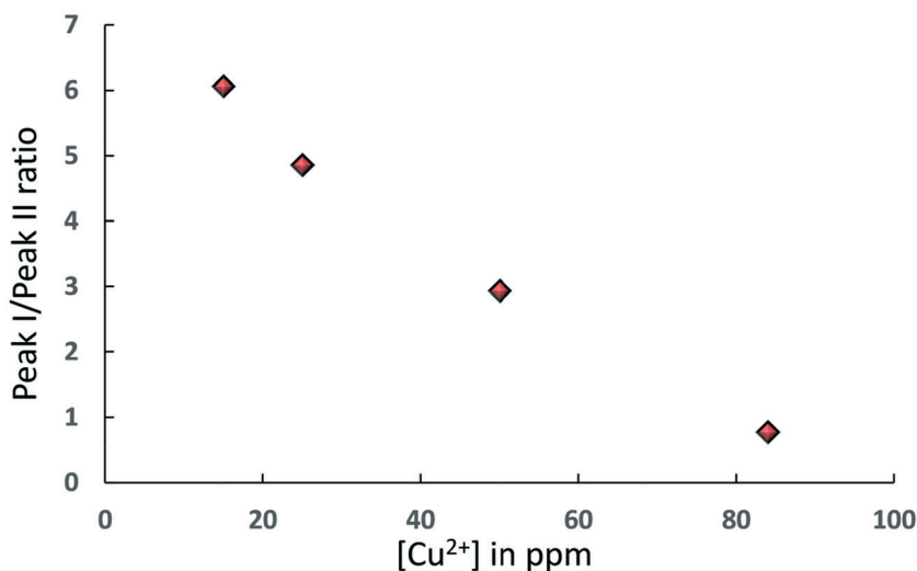
Fig. 4 Area ratio of peak I, associated to \text{Al}_2\text{O}_3 , over peak II, associated to \text{CuSO}_4 , as a function of [\text{Cu}^{2+}] for samples where both peaks are present in the T_1 – T_2 NMR correlation maps.
