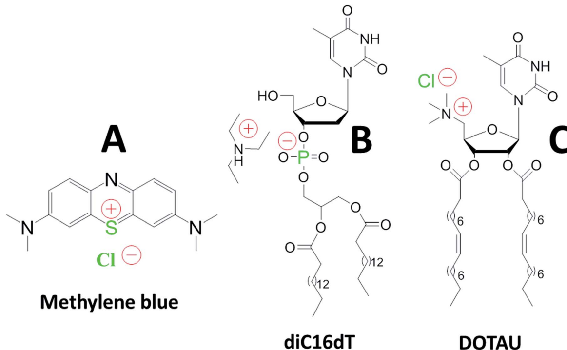
Fig. 1 Chemical structures of methylene blue (A), anionic nucleotide-lipid diC16dT a thymidine 3'-(1,2-dipalmitoyl- sn -glycero-3-phosphate) (B), cationic-nucleoside-lipid DOTAU (2',3'-dioleyl-5'-deoxy-5'-trimethyl-ammonium-uridine) (C). Green color highlight atoms identified with the EDX analysis (see Fig. 2c). Red color show molecules charges in solution.
