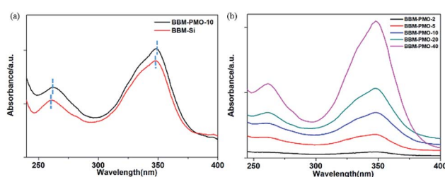
Fig. 4 UV-vis absorption spectra of (a) BBM-Si ( 10^{-5} M) and BBM-PMO-10 ( 10^{-4} g mL -1 ) in THF/H 2 O (3 : 7 v/v); (b) BBM-PMOs in THF/H 2 O (3 : 7 v/v, 10^{-4} g mL -1 ).
