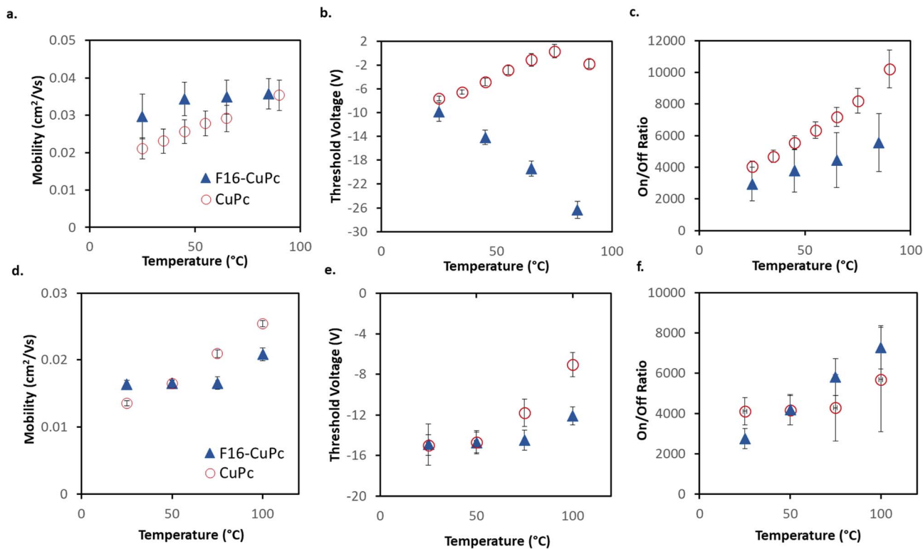
Fig. 4 Performance of BGBC CuPc and F 16 -CuPc devices (deposited at T = 140\text{ }^\circ\text{C} ) in air (a, b and c) or vacuum (d, e and f) at various temperatures. (a and d) Field-effect mobility. (b and e) Threshold voltage. (c and f) On/off ratio. Presented are the averages for four devices with error bars representing the standard deviation. The legend in (a and d) is the same as in (b and e) and (c and f). Devices were tested in the range of T = 25\text{ }^\circ\text{C} to T = 90\text{ }^\circ\text{C} in air, and T = 25\text{ }^\circ\text{C} to T = 100\text{ }^\circ\text{C} in vacuum.
