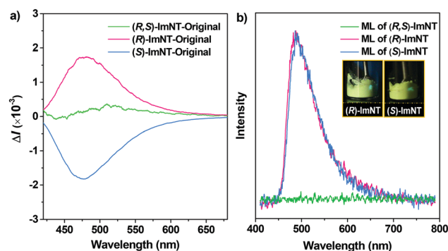
Fig. 3 CPL (a) and ML spectra (b) of the as-prepared samples of ( R,S )-ImNT, ( R )-ImNT and ( S )-ImNT under ambient conditions. The insets in (b) depict the ML images of ( R )-ImNT and ( S )-ImNT in daylight.
