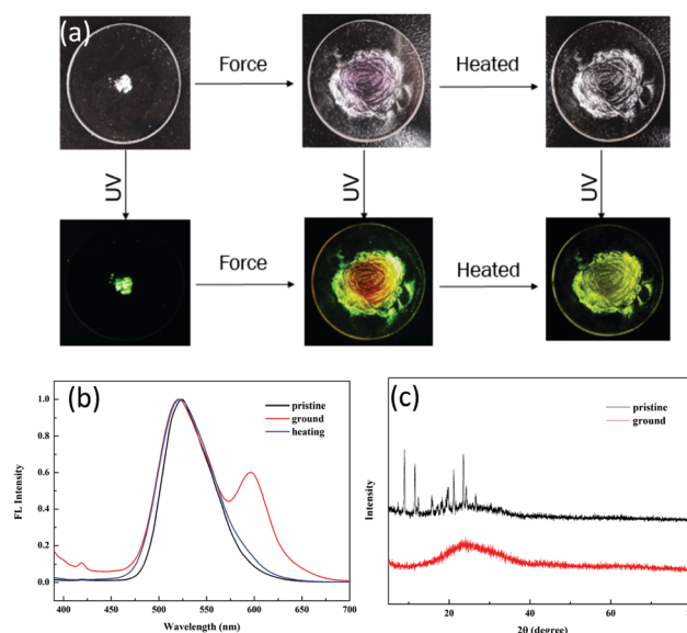
Fig. 4 (a) Optical images of the color-changing process of 1 due to shearing and heating under room light and 365 UV light. (b) Fluorescence spectra of the pristine powder, powder after heavy grinding and the heated powder. (c) XRD patterns of the pristine powder and powder after slight grinding.
