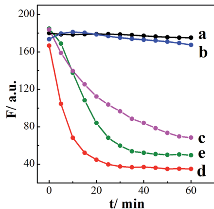
Fig. 4 Time-dependent fluorescence intensity changes of BDBA (a and d) and HBA (b and c) associated CDs in the absence (a and b) and presence (c and d) of H 2 O 2 , and time-dependent fluorescence intensity changes of the CDs incubated with H 2 Q (e).
