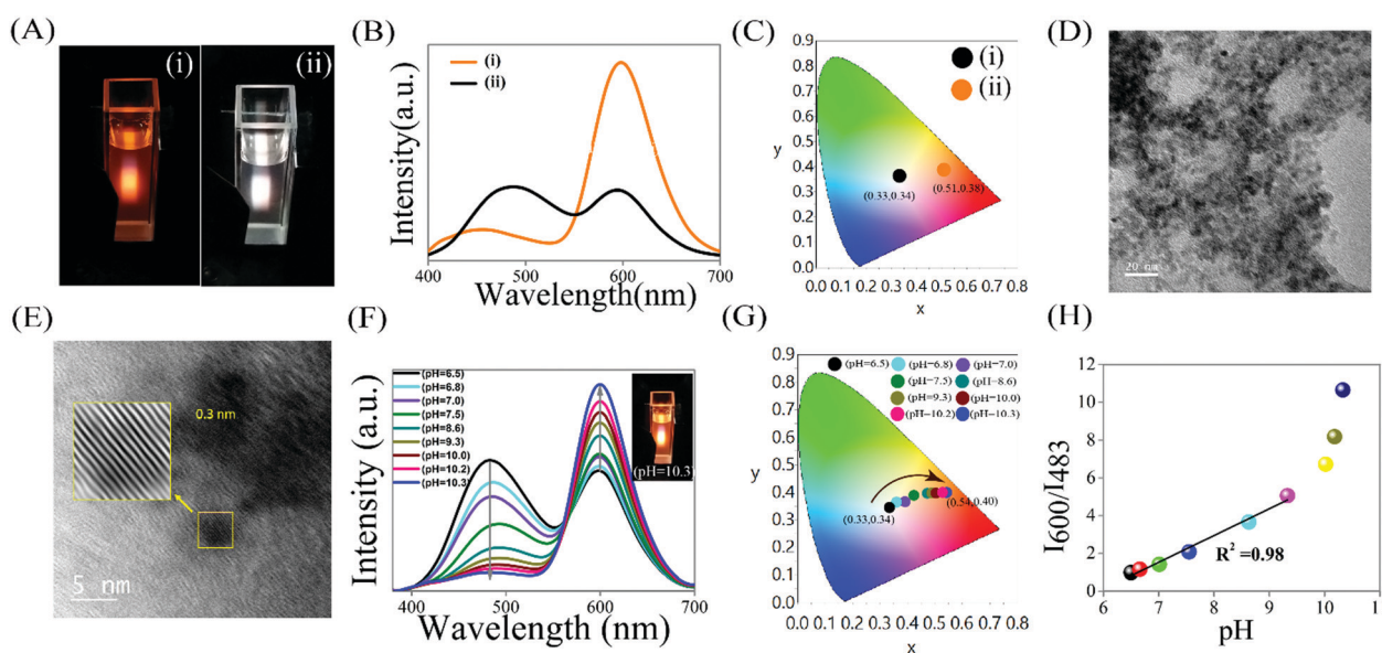
Fig. 1 (A) Digital photographs (B) emission spectra ( \lambda_{ex} = 330 nm) and (C) chromaticity color coordinates in CIE diagram of (i) Mn^{2+} doped ZnS QDs (pH 6.6) and (ii) WLE QDC (pH 6.5). (D) Transmission electron microscopy (TEM) image (scale bar = 20 nm), (E) high resolution TEM image (scale bar = 5 nm) and corresponding inverse fast Fourier transformed image (inset) of WLE QDC. (F) Emission spectra ( \lambda_{ex} = 330 nm) and (G) chromaticity color coordinates in CIE diagram of WLE QDC upon increasing their pH from 6.5 to pH 10.3. (H) Effect of pH (in the physiological range of 6.5–10.3) on the luminescence intensity ratio ( I_{600}/I_{483} ) of WLE QDC.
