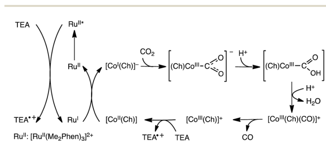
Scheme 13 Photocatalytic cycle for two-electron reduction of CO 2 to CO with a cobalt(II) chlorin complex (Co I (Ch)) adsorbed on multi-walled carbon nanotubes (Co I (Ch)/MWCNTs). Reprinted with permission from ref. 150. Copyright 2016, Royal Society of Chemistry.
