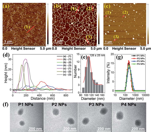
Fig. 2 AFM images of P3 NPs formed at r 0 (a), 1 (b), and 30 (c). (d) The height cross-section along the lines shown with numbers in panels (a–c). (e) Size distribution of P3 NPs ( r = 30) shown in (c), determined using AFM. (f) TEM images of the P1–P4 NPs ( r = 30). (g) DLS analysis of the P1–P4 NPs ( r = 30).
