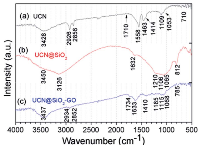
Fig. 6 FTIR spectra of (a) UCNs, (b) UCN@SiO 2 NPs and (c) UCN@SiO 2 -GO nanocomposite.
