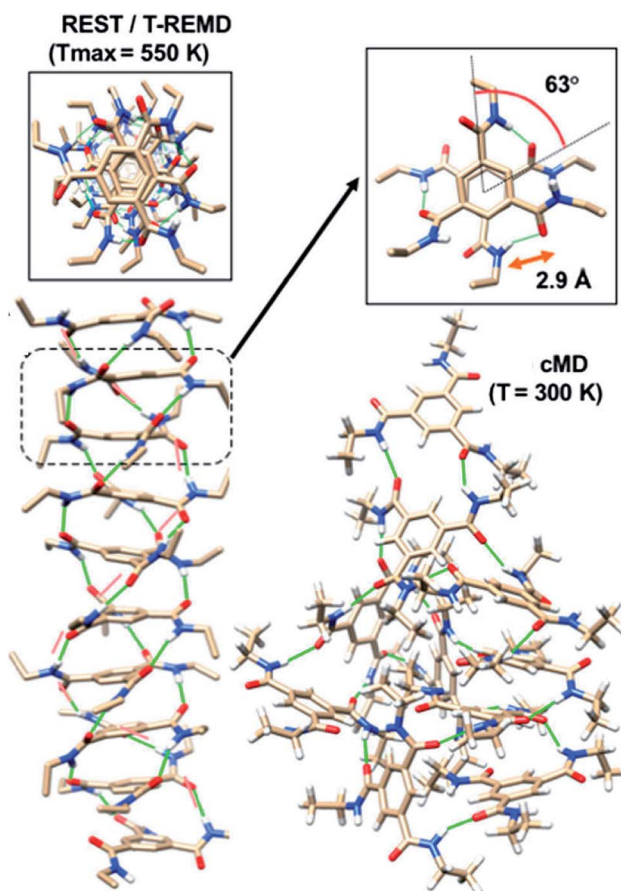
Fig. 15 Self-assembled structures from common MD (cMD), T-REMD and REST at different values of T_{max} . This figure has been reproduced from ref. 87 with permission from the American Institute of Physics.
