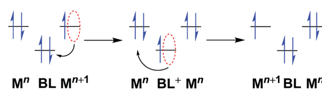
Fig. 4 Bridging ligand-mediated electron transfer and hole transfer pathways in mixed valence complexes. 19c,d
