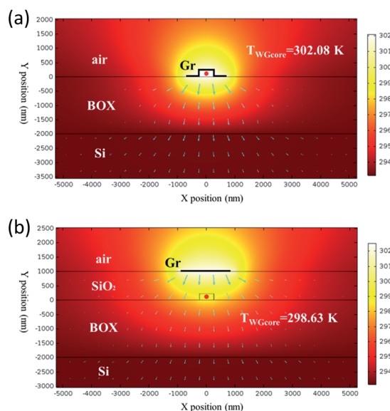
Fig. 4 Simulated thermal field distribution of the proposed structure with graphene contact heating (a) and the conventional structure with 1 \mu\text{m} -thick top SiO 2 cladding layer (b). Blue arrows shows the directions of heat flux.
