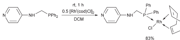
Scheme 19 The reaction of phosphinodiphenylamine ligands with [\text{Rh}^{\text{I}}(\text{cod})\text{Cl}]_2 .
