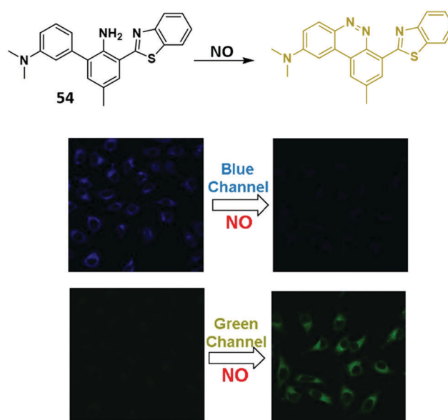
Scheme 50 An ESIPT fluorescent probe 54 for the ratiometric detection of NO via formation of a benzo[c]cinnoline derivative. Measurement conditions: PBS buffer (1.0 mM, pH = 7.4). Reproduced with permission from ( Sens. Actuators, B , 2018, 259 , 347–353). Copyright (2018) Elsevier.
