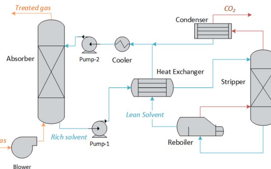
Fig. 1 Process flow diagram of the CO 2 absorption capture plant modelled in this work.
