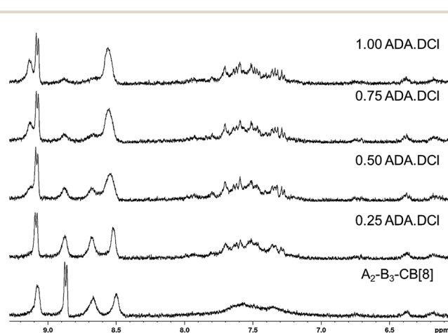
Fig. 4 ^1\text{H} NMR spectra in \text{D}_2\text{O} of \text{A}_2\text{-B}_3\text{-CB[8]} hyperbranched supramolecular polymer upon titration with up to 1 molar equivalent of ADA·DCl relative to CB[8].
