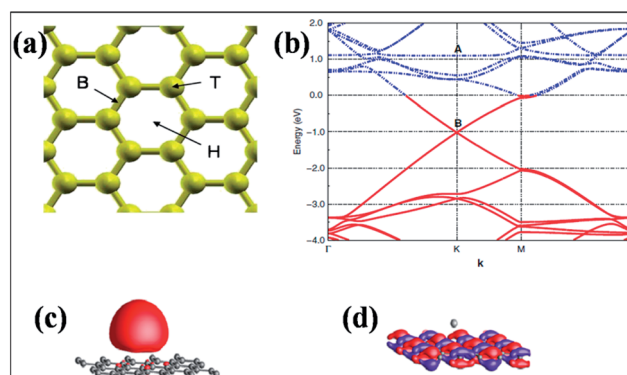
Fig. 5 (a) Adsorption sites on the surface of graphene: hollow (H), bridge (B), and top (T). Reproduced with permission. 65 © 2008 American Physical Society. (b) Band structure representation of K-adsorbed graphene in the vicinity of the Fermi energy. The Fermi level is set to zero. Occupied states are shown by red lines, while empty levels are shown by blue lines. The unoccupied bands of pristine graphene around B became occupied due to the adsorption. (c, d) Representations of the real part of the wave functions of the electronic levels, marked as A and B in panel (b). The wave function of the level marked as A is localized on the K atom, while the wave function of the occupied level, which is marked as B, is delocalized over the hexagonal graphene layer. Reproduced with permission. 75 © 2010 American Physical Society.
