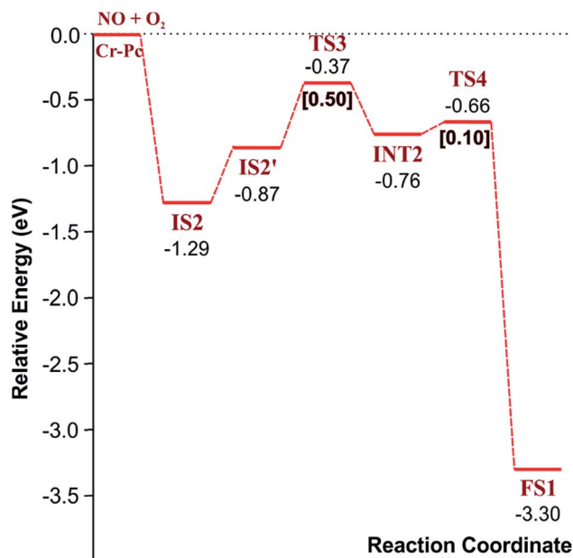
Fig. 6 Reaction pathway of the LH mechanism for the first NO 2 production.
