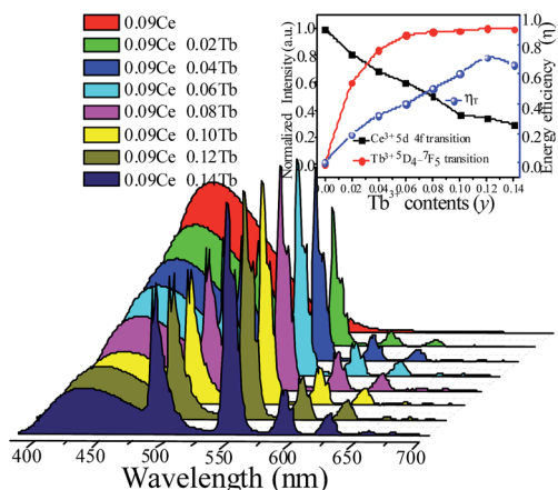
Fig. 7 PL spectra for LSN:0.09Ce 3+ ,yTb 3+ phosphors on Tb 3+ doping content (y) excited at 360 nm. The inset shows the emission intensity of Ce 3+ and Tb 3+ with different Tb 3+ contents and energy transfer efficiency on changing Tb 3+ contents.
