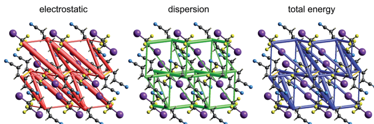
Fig. 14 1,4-Dicyanobutane:1,2-diiodo-1,1,2,2-tetrafluoroethane co-crystal (EBIHIH): energy frameworks for separate electrostatic (red) and dispersion (green) contributions to the total nearest neighbour pairwise interaction energies (blue). See Fig. 10 for details.
