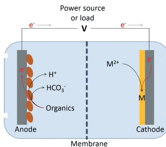
Fig. 4 Illustration of a microbial electrochemical reactor with a microbial anode oxidizing organics and an abiotic cathode reducing metal ions.
