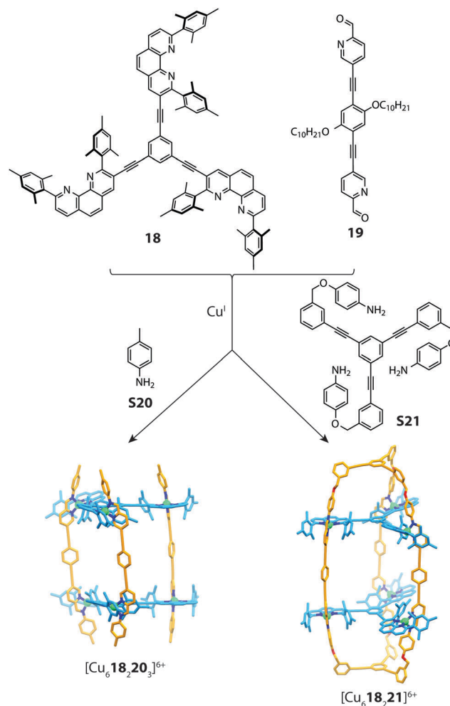
Fig. 13 Self-assembly of a [\text{Cu}_6\text{18}_2\text{20}_3]^{6+} prism (mediated by S20 ) and a doubly-partitioned cage [\text{Cu}_6\text{18}_2\text{21}]^{6+} mediated by S21 .
