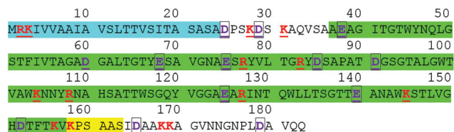
Fig. 4 Full sequence of streptavidin from the work of Argarana et al. B1 the blue region (1–24) corresponds to the N-terminus signalling region that is likely removed in vivo . 76 The green highlighted region (37–157) corresponds to the truncated-structure that was resolved in the X-ray crystal structure published by Weber et al. 21 (PBD ID: 1STP) and used in the simulation of net charges presented here. Pähler et al. B2 truncated streptavidin such that residues residues 37–163 were present ( i.e. green and yellow regions). At pH 7, residues that based on the intrinsic pK_a of the individual amino acid are usually positively charged (red) or negatively charged (purple, black box outline) are both underlined. This analysis shows, for example, that the streptavidin used by Weber et al. is likely to be 1 q more negative than the net charge of the streptavidin of Pähler et al. , due to the positive lysine residue (K) labelled 160 in the figure. Weber et al. comment that the termini are likely flexible or disordered, 21 suggesting that the intrinsic pK_a of the amino acids for the non-highlighted regions are reliable as they are not buried within the protein.
