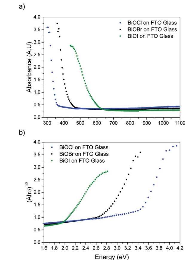
Fig. 5 (a) UV/vis spectra of BiOX ( X = \text{Cl, Br, I} ) films deposited on FTO glass and (b) corresponding Tauc plots.
