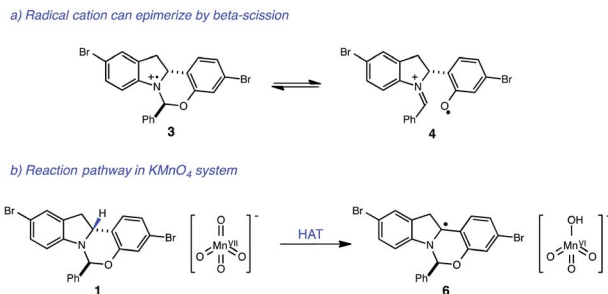
Fig. 3 (a) Proposed pathway for epimerization of starting material. (b) Proposed mechanism for KMnO 4 -mediated oxidation of indoline core.
