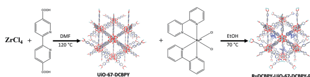
Scheme 3 RuDCBPY–UiO-67–DCBPY-PS.
