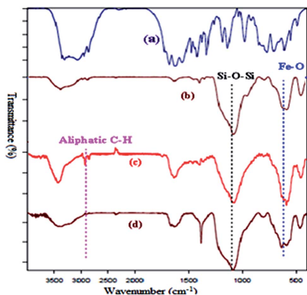
Fig. 1 FT-IR spectra of pure L-arginine (a), \text{Fe}_3\text{O}_4 @ \text{SiO}_2 (b) \text{Fe}_3\text{O}_4 @ \text{SiO}_2 @ \text{L-arginine} (c) and Cu(II) immobilized on \text{Fe}_3\text{O}_4 @ \text{SiO}_2 @ \text{L-arginine} (d).
